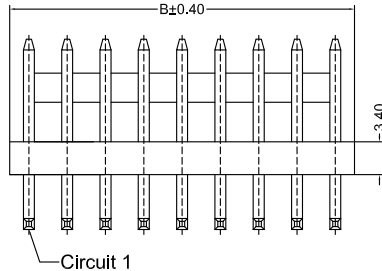
Circuit 1
